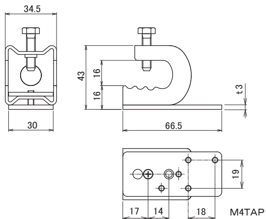
S-UB34 (レクト40/30/24 共通)
