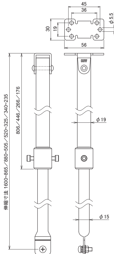
S-105/106/107/107-SS (レクト40/30 共通)
