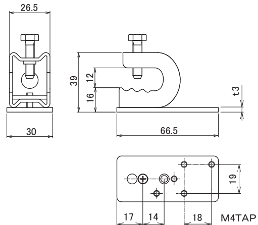
S-UB43 (レクト40/30/24 共通)
