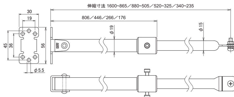
S-105/106/107/107-SS (レクト40/30 共通)
