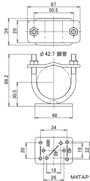
S-UB43 (レクト40/30/24共通)
