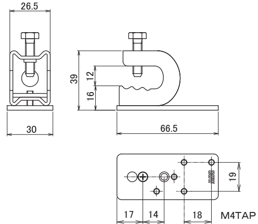
S-UB43 (レクト40/30/24共通)
